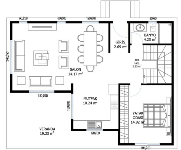
ZEMİN KAT PLANI 100 m 2
