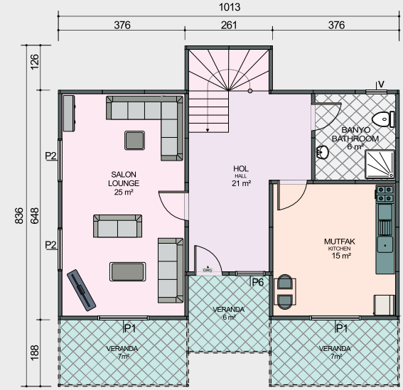
Zemin Kat Planı / Ground Floor Plan 66 m 2 + 20 m 2 = 88 m 2
